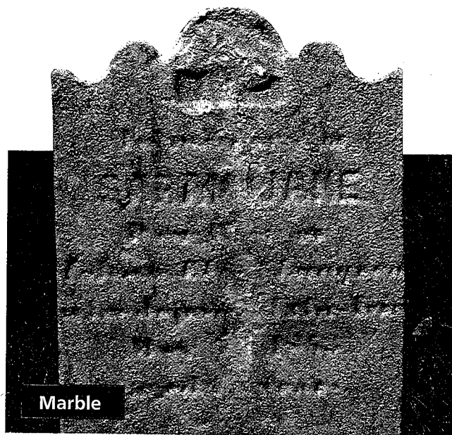
FIGURE 5 Which Rock Weathers Faster? These two tombstones are about the same age and are in the same cemetery, yet one has weathered much less than the other. Inferring Which type of stone weathers faster, granite or marble? Explain.
