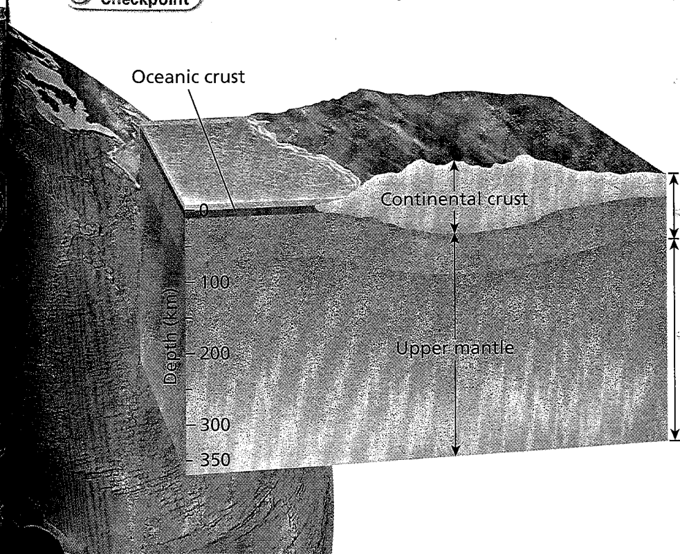
FIGURE 6 Lithosphere and Asthenosphere The rigid lithosphere, which includes the crust, rests on the softer material of the asthenosphere.
