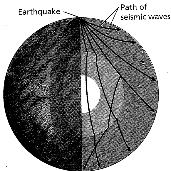
FIGURE 3 Seismic Waves
